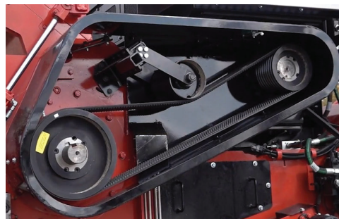
Adjustable backside flat idler allow the operator to adjust drive belt tensioning with no need to move the engine.
