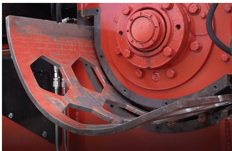
Single, side-load grate system and single side-load anvil allow for single-person removal.
