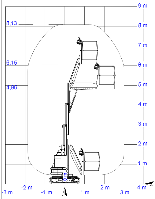
The spacious steel basket allows for two operators to work both indoors and outdoors and can safely elevate on slopes of up to 5°!
